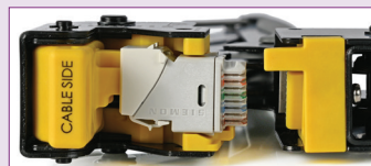
Salida/Outlet Keystone
